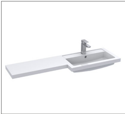
1200mm POLYMARBLE BASIN & WORKTOP 600mm one taphole basin / 600mm worktop 1202.5mm x 355/255mm, right hand WE-120RHPB
