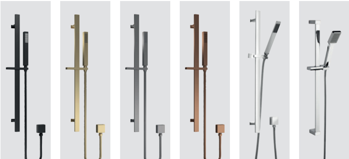
Slide Rail Kit Matt Black. Brass. Outlet Elbow included. H685mm A4167 £425.00 LP Slide Rail Kit Brushed Brass. Brass. Outlet Elbow included. H685mm A8167 £425.00 LP Slide Rail Kit Brushed Pewter. Brass. Outlet Elbow included. H685mm A7167 £425.00 LP Slide Rail Kit Brushed Bronze. Brass. Outlet Elbow included. H685mm A15167 £425.00 LP Rectangular Slide Rail Kit Brass. Outlet Elbow included. H685mm A3167 £259.00 LP1 Rectangular Slide Rail Kit Brass/ABS. Outlet Elbow not included. H700mm STY059 £113.00 LP1
