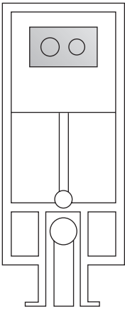
Dual Flush Concealed WC Cistern with Wall Hung Frame H1136-1336 x W520mm Flush Plate with Round Buttons ● Chrome XTY007S £364.00 ● White XTY107S £367.00 ● Black XTY407S £381.00 ● Brass XTY807S £410.00
