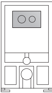
Mid-Height Dual Flush Concealed WC Cistern with Wall Hung Frame H890-1090 x W520mm Flush Plate with Round Buttons ● Chrome XTY007R £364.00 ● White XTY107R £367.00 ● Black XTY407R £381.00 ● Brass XTY807R £410.00
