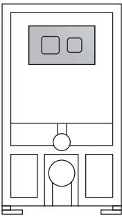
Mid-Height Dual Flush Concealed WC Cistern with Wall Hung Frame H890-1090 x W520mm Flush Plate with Square Buttons ● Chrome XTY007S £364.00 ● White XTY107S £367.00 ● Black XTY407S £381.00 ● Brass XTY807S £410.00
